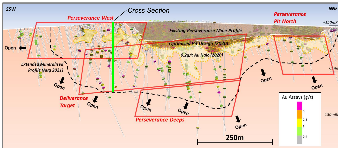
Perseverance Mine Long Section with 2020 0.2 g/t Au Halo & New 2021 Profile Extensions 1
